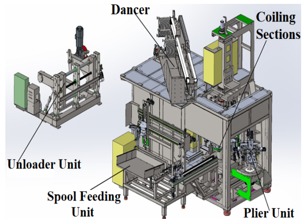
Fig. 6. Sections of the 3-headed spool-coil winding machine with increased capacity
