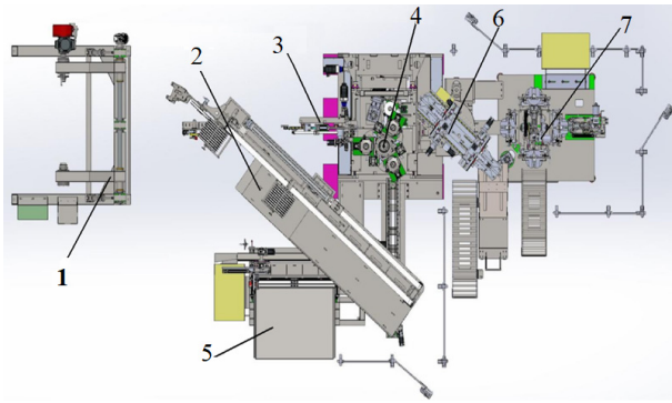
Fig. 2. Machine General View 1. Unloader Unit 2. Dancer 3. Traverse Unit 4. Coiling Section 5. Spool Feeding Unit 6. Packaging Unit 7. Main Control Panel
