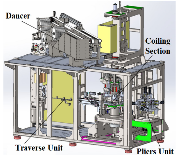
Fig. 5. Sections of the 3-headed spool-coil winding machine with increased capacity
