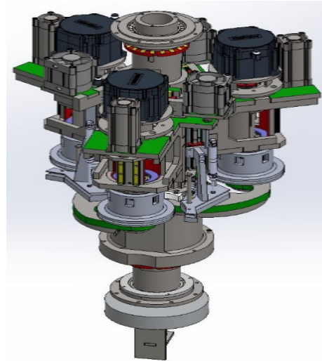
Fig. 3. Coiling Section
