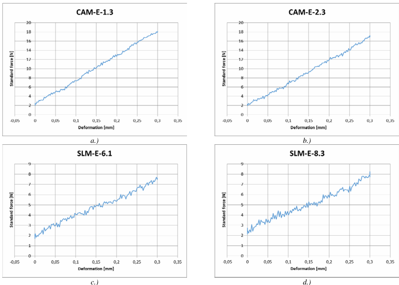
Fig. 2. Bending stress-strain plots of titanium alloy specimens used to determine modulus of elasticity. Milled alloy before – a) and after – b) heat treatment and SLM alloy before – c) and after – d) heat treatment
