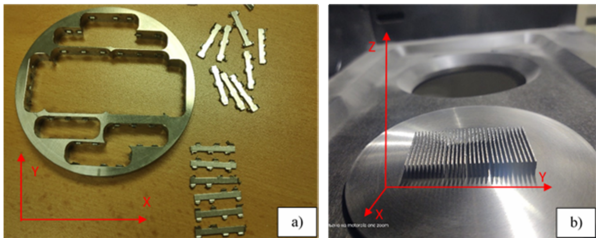
Fig. 1. Ti6Al4V alloy disc with milled samples – a) and disposition of the samples on the working table of SLM machine – b)
