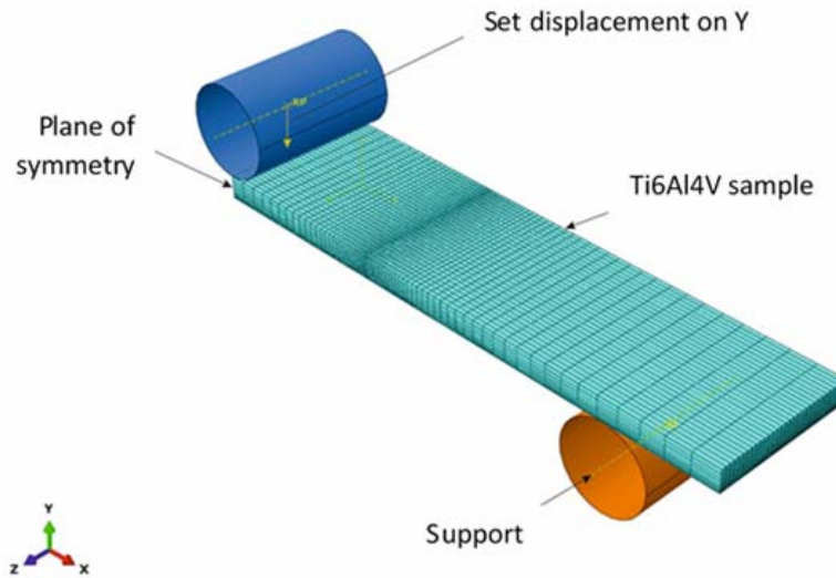
Fig. 3. FE model for determining the modulus of linear deformations of TiAl6V4 alloy
