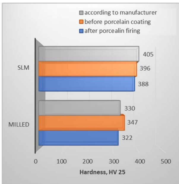
Fig. 4. Micro-hardness of Ti6Al4V alloy
