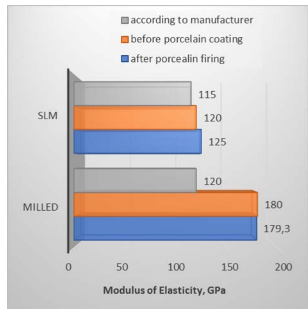
Fig. 5. Modulus of elasticity of Ti6Al4V alloy
