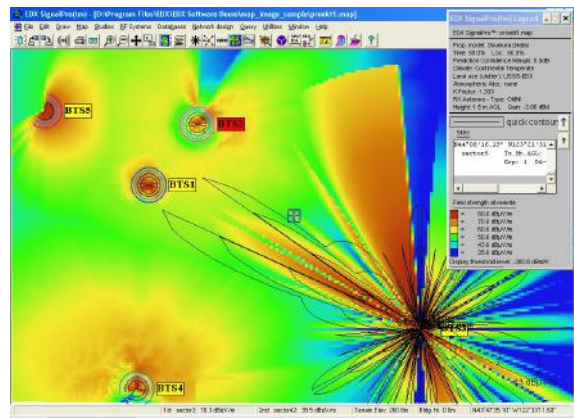
Fig. 6. Levels of field intensity in dBµV (minimum permissible level – 43dBµV/m)
